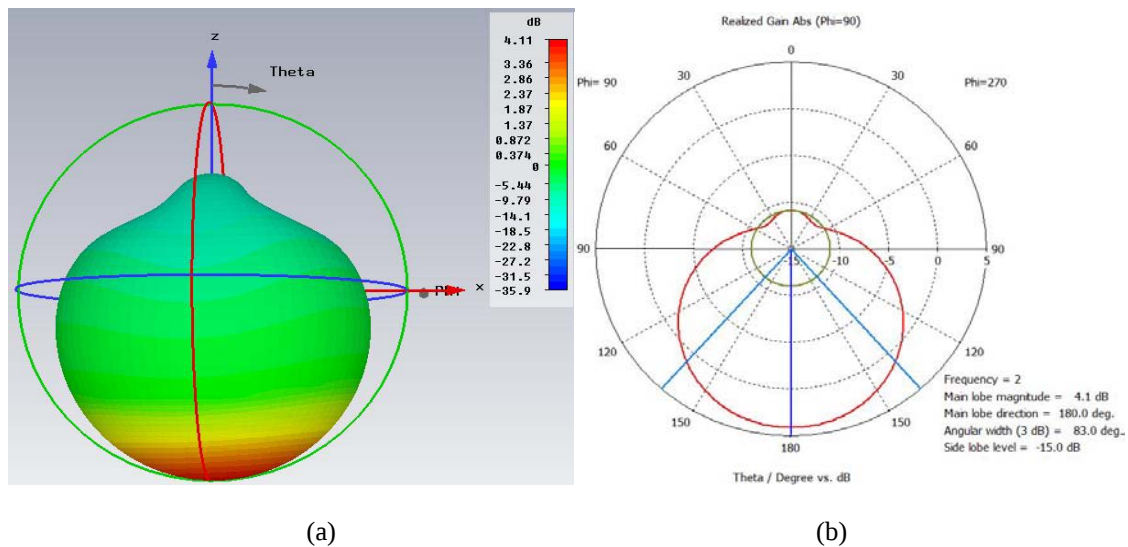
Fig. 13: Simulated (a) three dimension and (b) two dimension radiation pattern of the multilayer structure designed at 2 GHz
