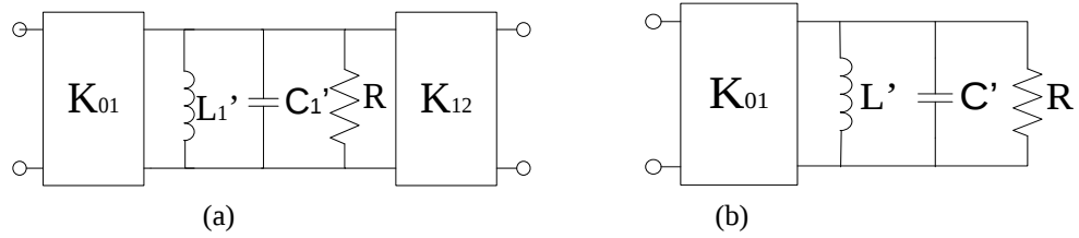
Fig. 3: Single-mode circuit of (a) rectangular SIW filter and (b) rectangular microstrip patch antenna
